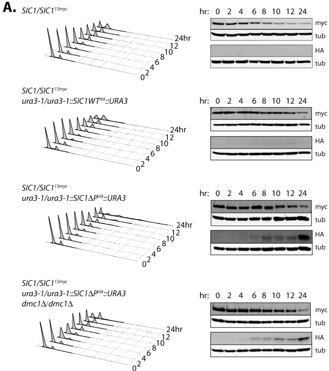
Figure 22. Heterozygote SIC1 13myc reveals no change in endogenous Sic1 protein level between HOP1pr::SIC1Δ PHA and HOP1pr::SIC1Δ PHA with dmc1Δ .
