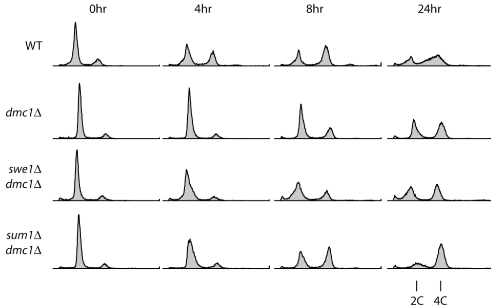
Figure 20. Mutations in Swe1 and Sum1 do not bypass dmc1Δ -induced arrest by DAPI staining.
